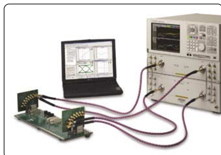
The Agilent N1957B Physical Layer Test System is used for 4-port 50 GHz signal integrity measurements
